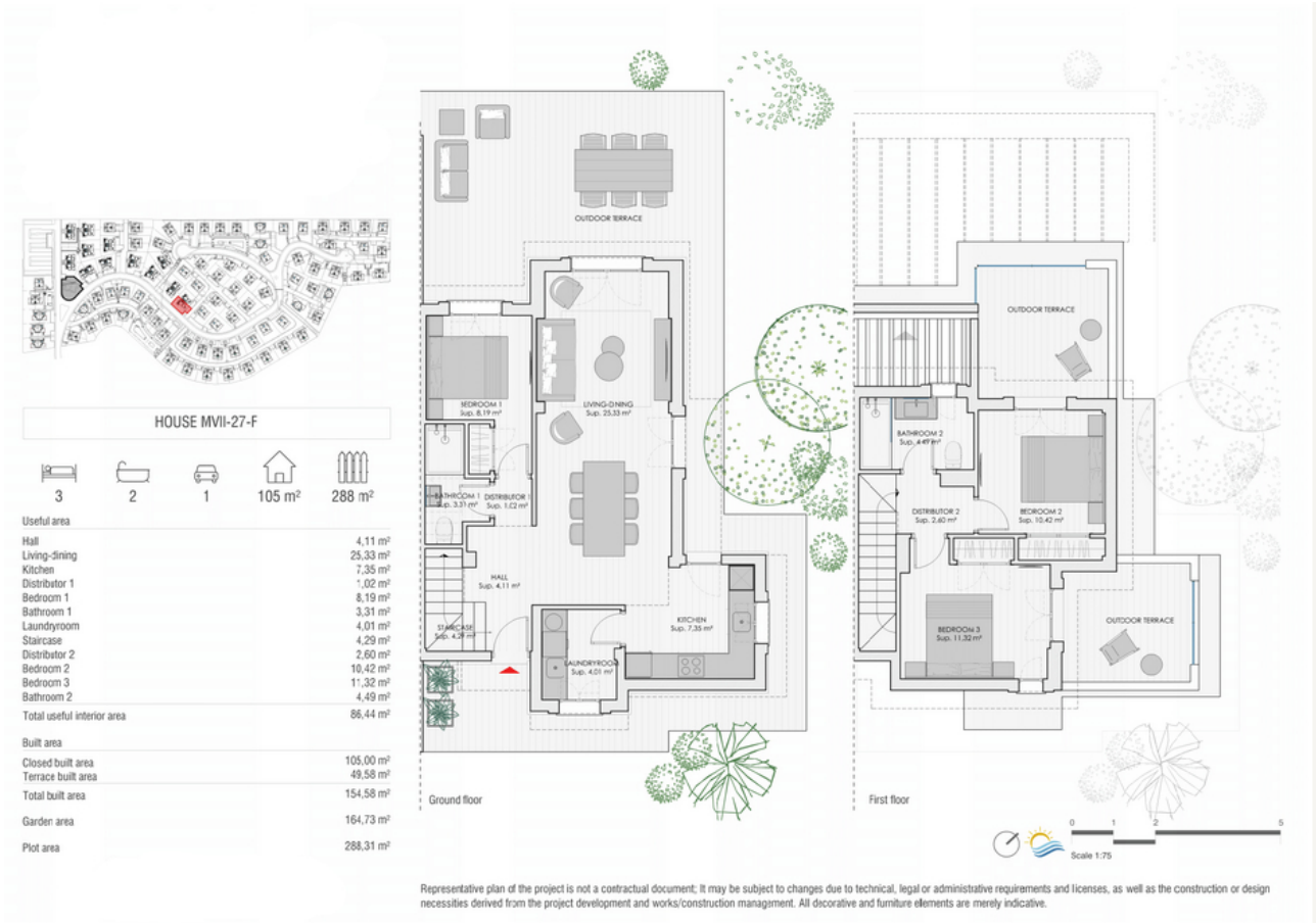
Floorplan MVII-27-F
