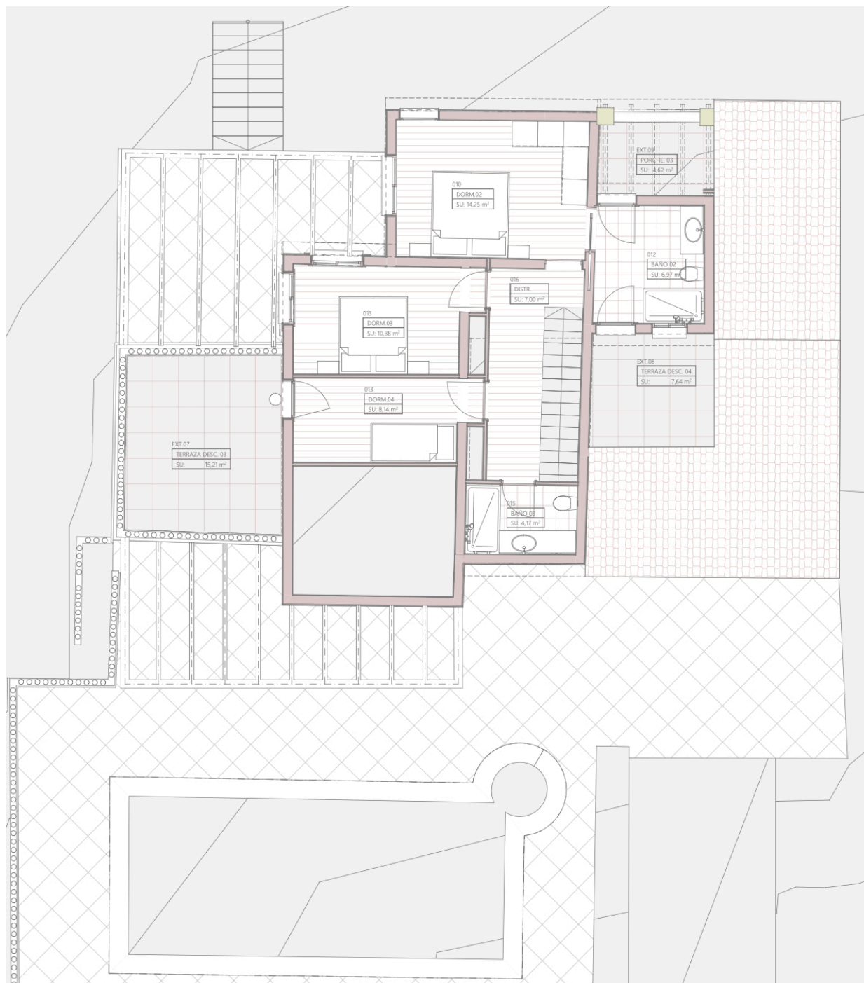
Floorplan First Floor
