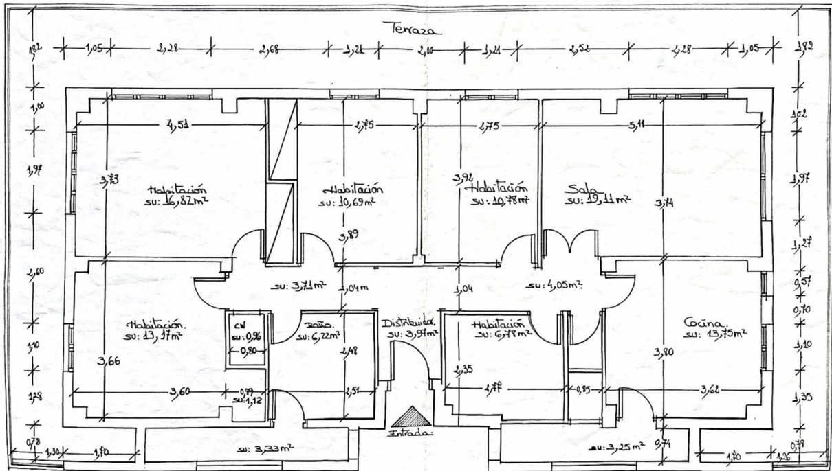
Floorplan
